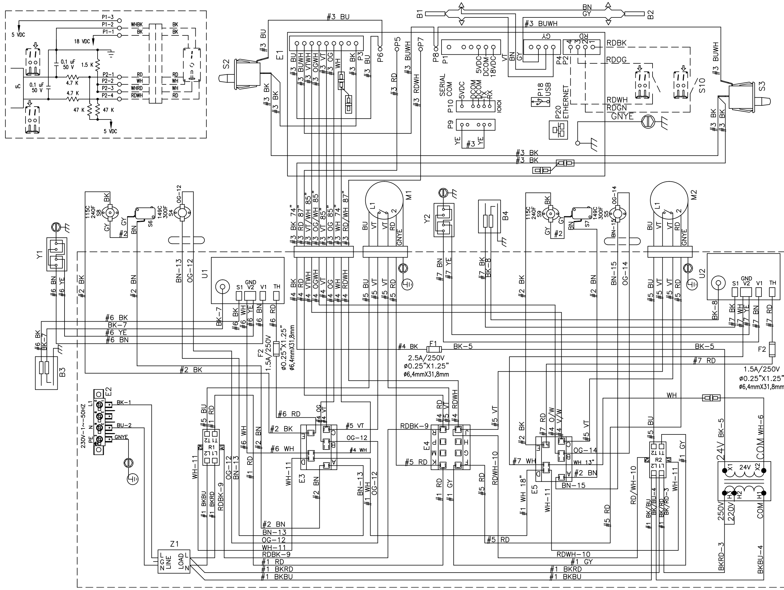
9506-648-001A WIRING DIAGRAM DC50X2N-59CC_X
