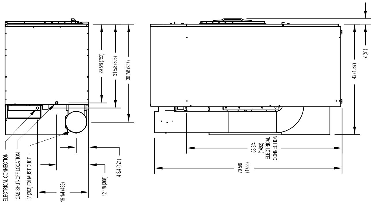
T30 COMMERCIAL DRYER MOUNTING DIMENSIONS
