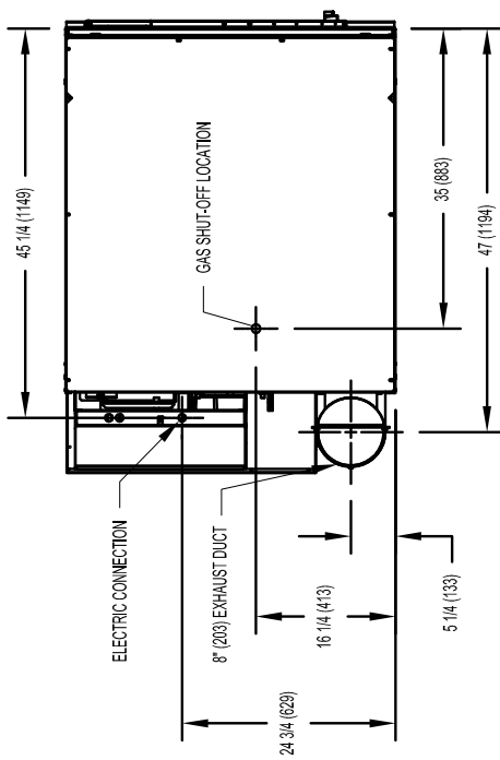
T80 COMMERCIAL DRYER MOUNTING DIMENSIONS
