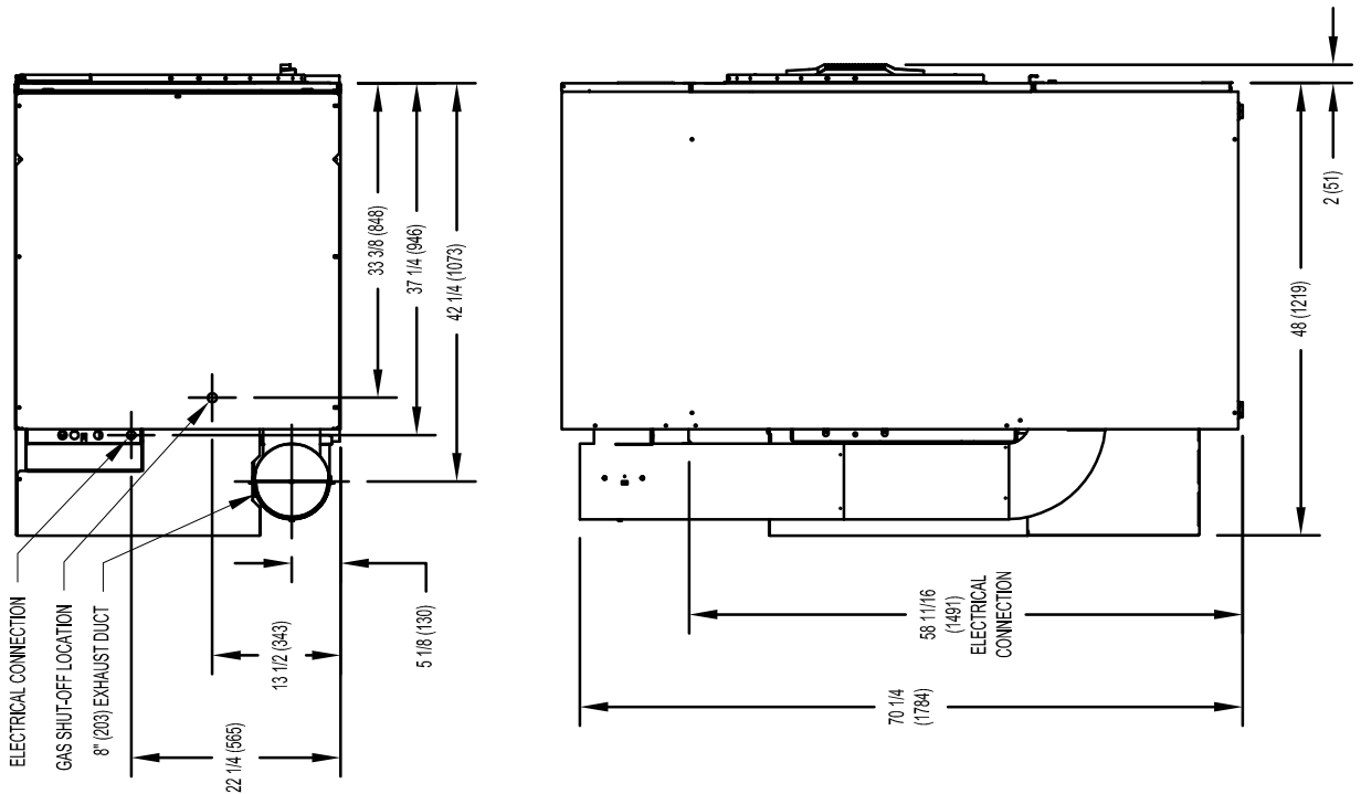
T50 COMMERCIAL DRYER MOUNTING DIMENSIONS
