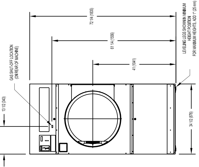
T50 COMMERCIAL DRYER MOUNTING DIMENSIONS
