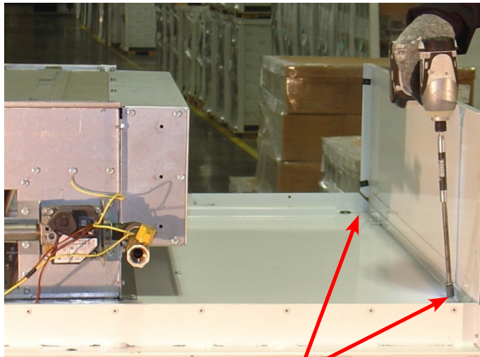
5/16 head screws
