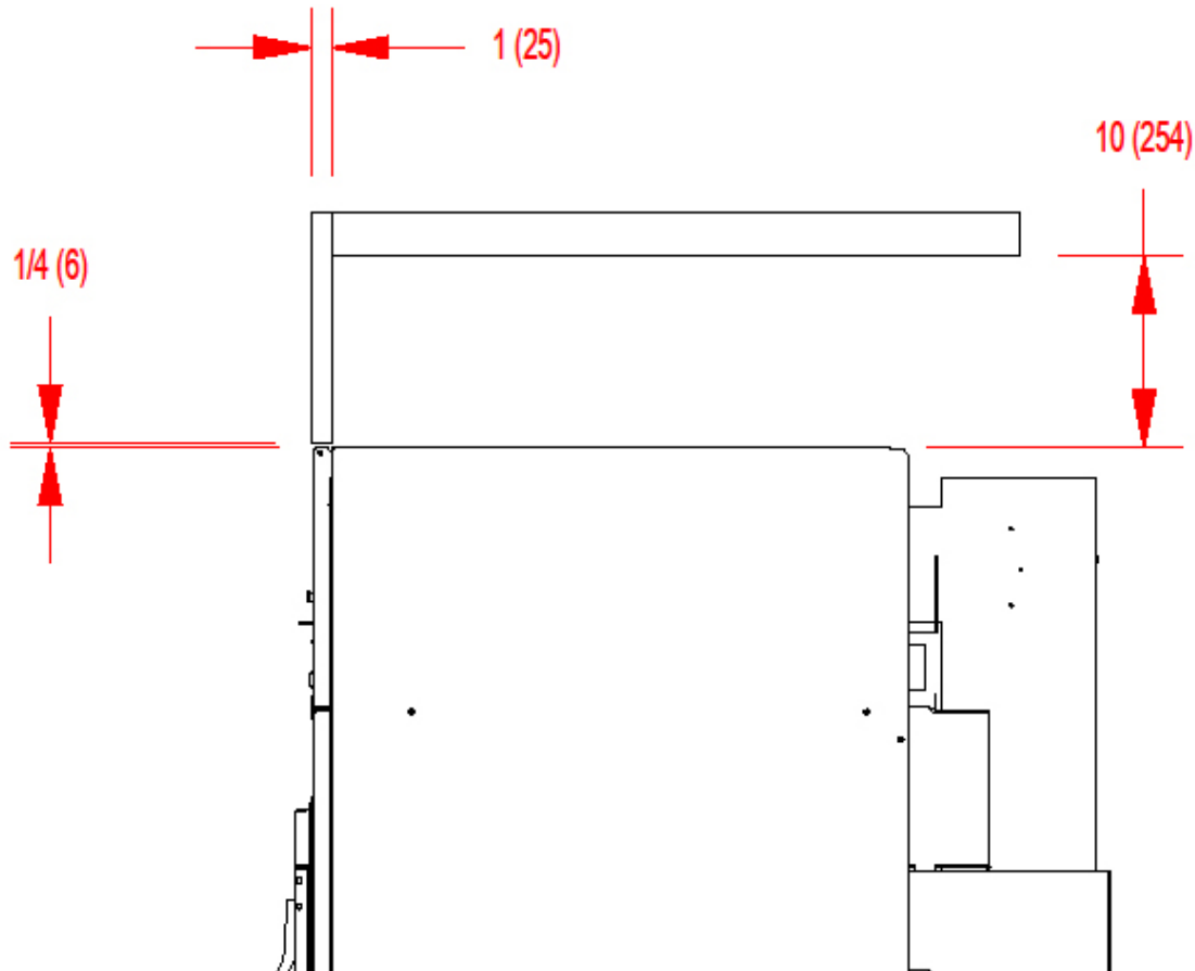
VERTICAL CLEARANCE DIMENSIONS - ALL C Series (30/50/80/120)
