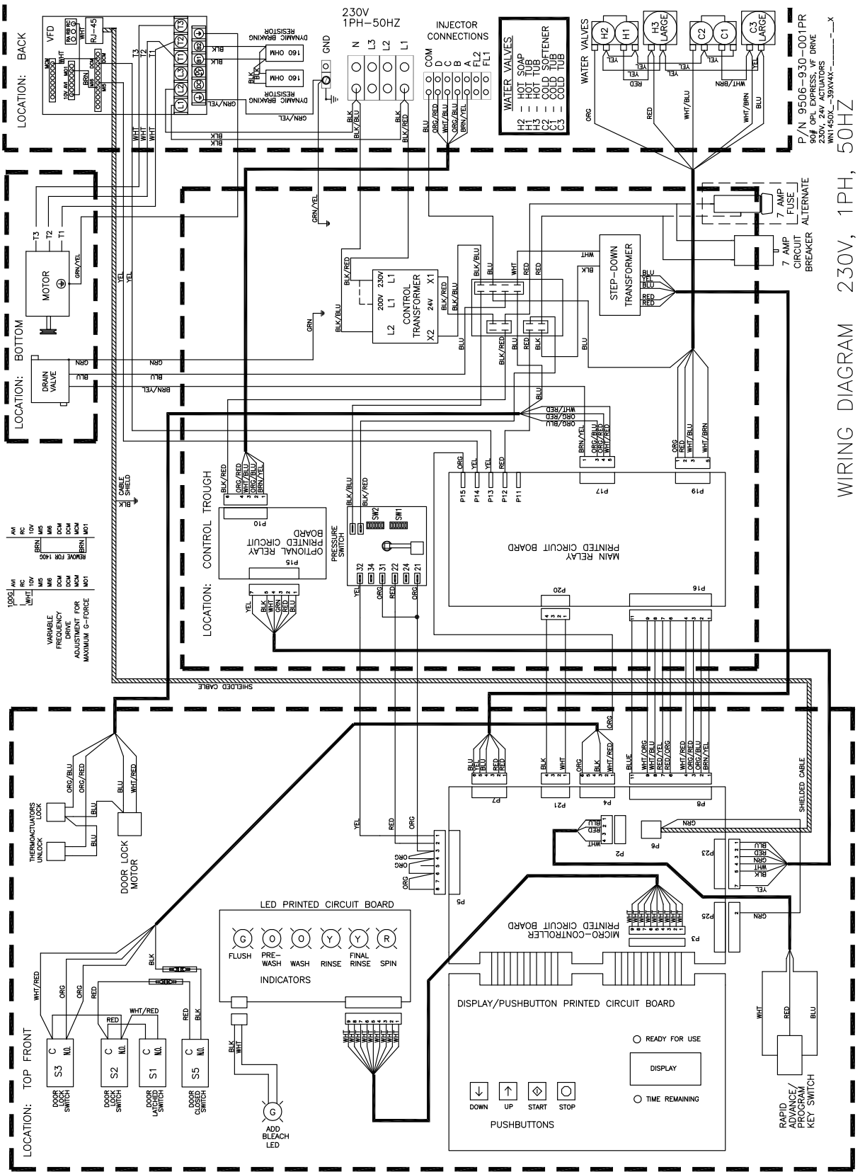
T-1450-39 Diagram V4
