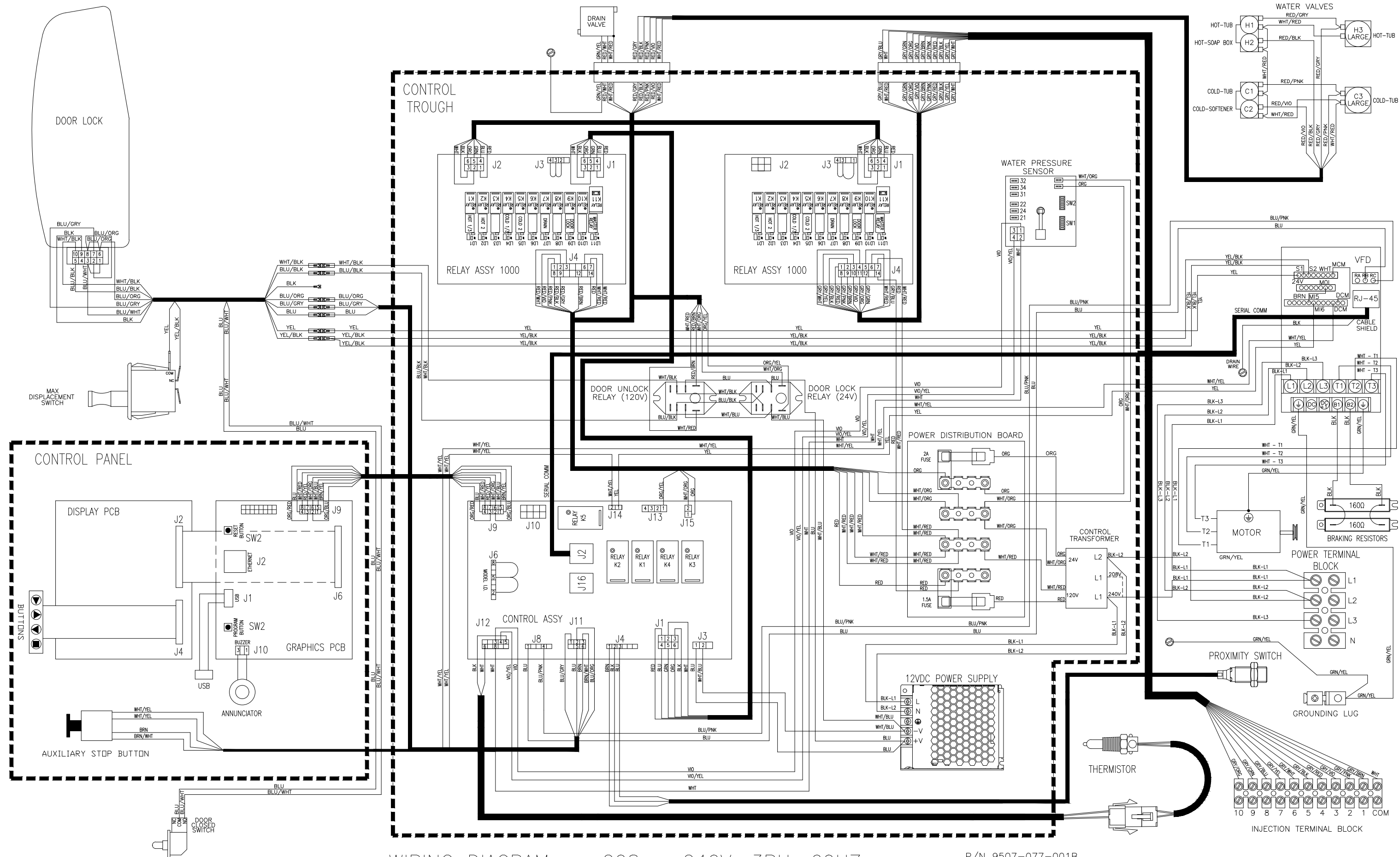
WIRING DIAGRAM 208 - 240V, 3PH, 60HZ
