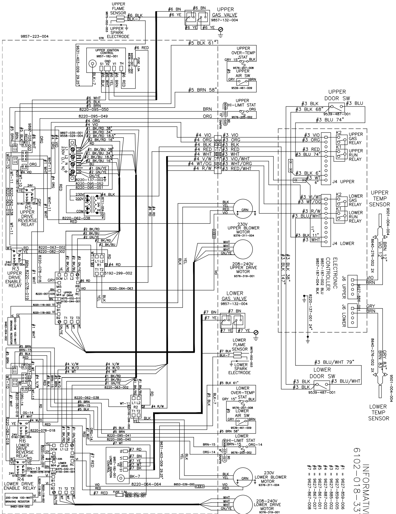
9506-805-001PR WIRING DIAGRAM DN50X2NC-39_B_R
