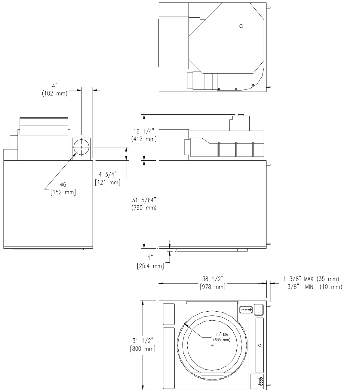
FIGURE 1- Dryer Dimensions
