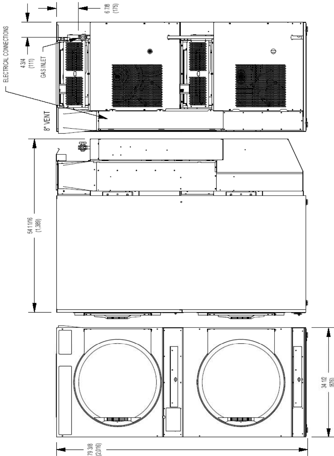
Figure1, 50# Stack Dryer Dimensions, Inches (mm)
