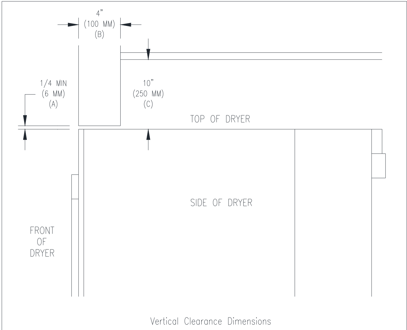
FIGURE 2 - VERTICAL CLEARANCE DIMENSIONS
