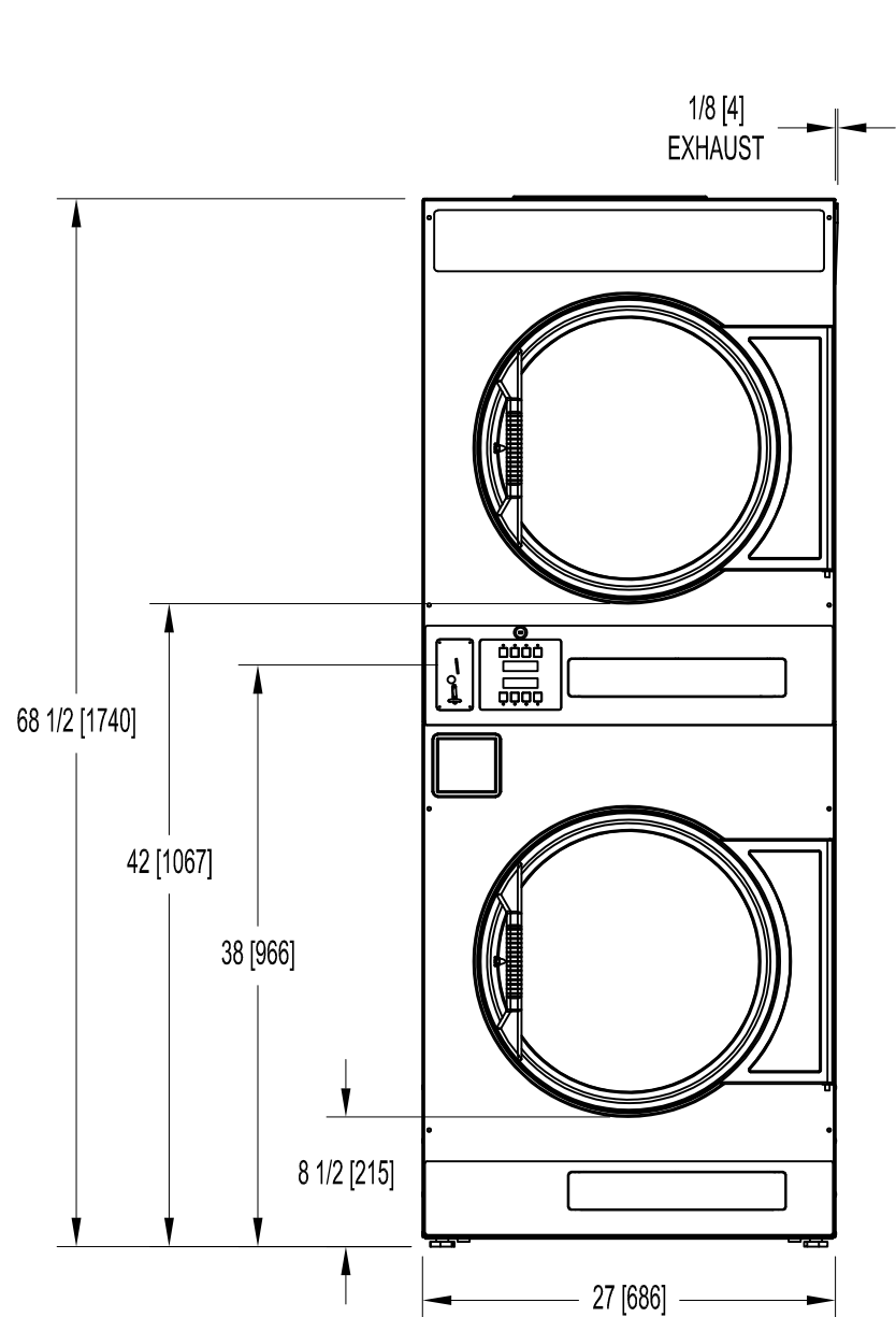
DIMENSIONS ARE IN INCHES [MILLIMETERS]
